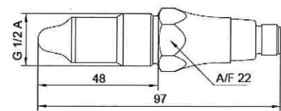
LBFS-xx4xx.x G 1/2 A hygienerecht
