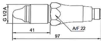
LBFS-xx1xx.x G 1/2 A ISO 228-1
