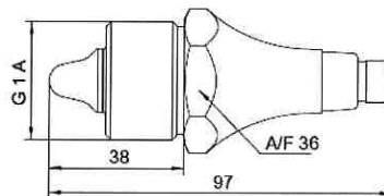
LBFS-xx3xx.x G 1 A ISO 228-1
