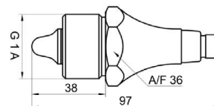
LBFS-xx3xx.x G 1 A ISO 228-1 (BCID: G11)
